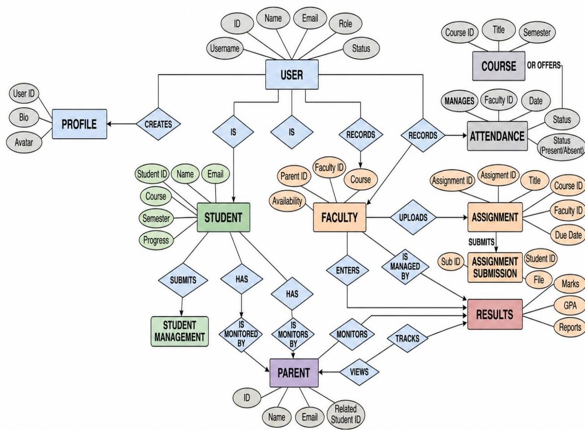
Entity-Relationship (ER) Diagram: Online Learning Portal (OLP)
